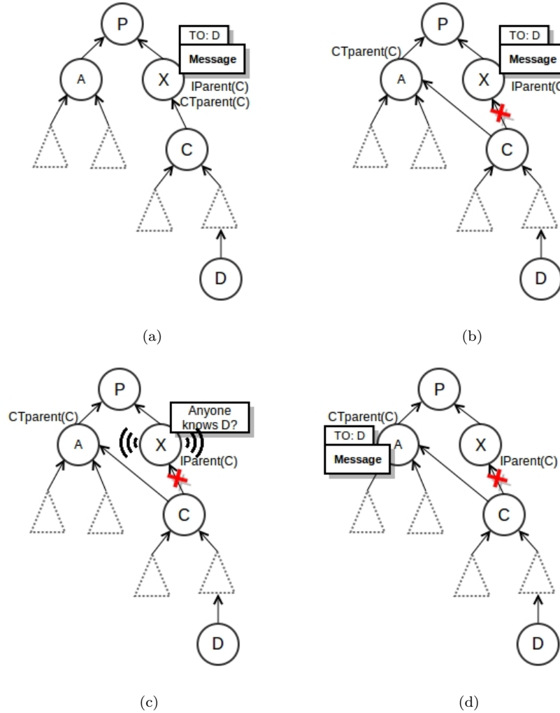
Figure 4: Alternative top-down routing upon Ctree change.
